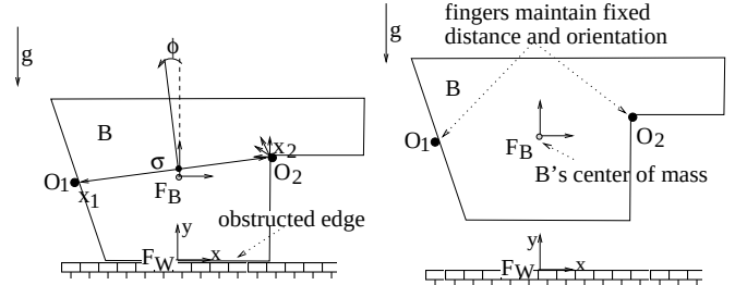
Fig. 1: A polygonal object \mathcal{B} supported by point fingers \mathcal{O}_1 and \mathcal{O}_2 in a basket grasp (the full robot hand is not shown). The parameter \sigma describes the inter-finger distance, \phi measures the two-fingers' orientation relative to gravity.
