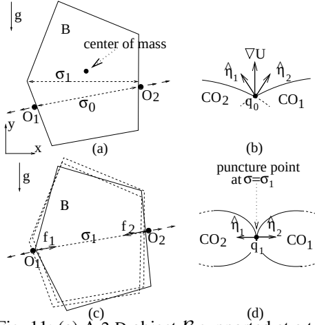
Fig. 11: (a) A 2-D object B supported at a two-finger basket grasp with inter-finger distance \sigma_0 . (b) Cross section of (q, \sigma) \in \mathbb{R}^4 at the basket grasp point (q_0, \sigma_0) . (c) The critical drop-off finger opening, \sigma_1 , is a frictionless two-finger equilibrium grasp of B . (d) Cross section of (q, \sigma) \in \mathbb{R}^4 at the drop-off puncture point (q_1, \sigma_1) .
